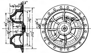
Figs. 920-921. Front Head. Cylinder Heads, Atlantic (4-4-2) Locomotive. Pennsylvania Railroad.
